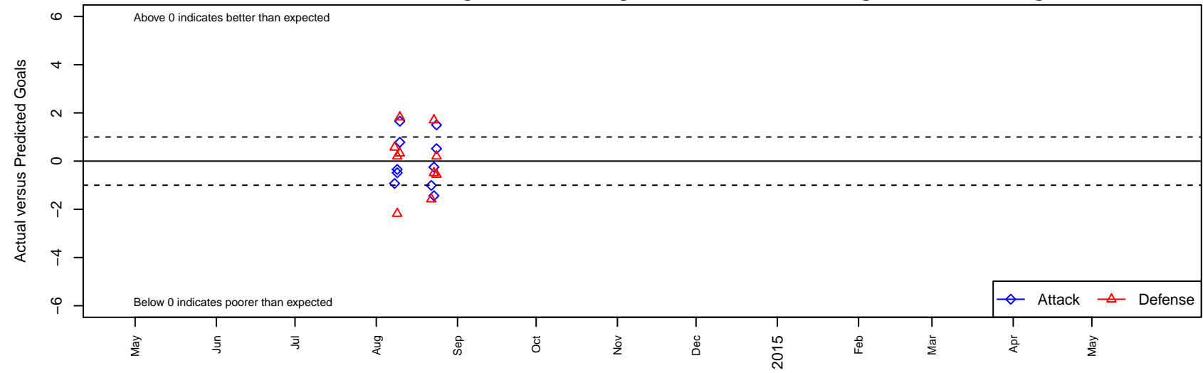
Washington Timbers Warriors B99 Dots are actual minus expected GF (blue circles) and GA (red triangles). Blue line is smoothed change in attack strength. Red is smoothed change in defense strength.
